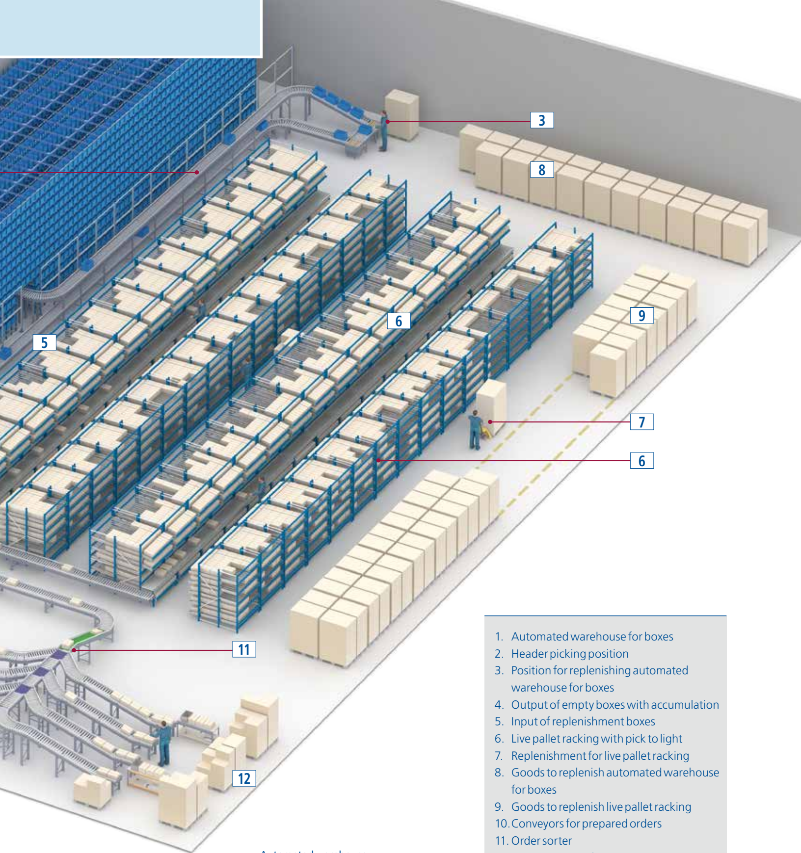
Automated warehouse for boxes combined with live pallet racking and an order sorter.
