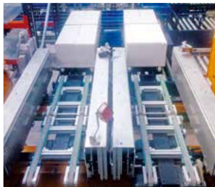
Cradle with two extractors that carries four boxes at once.
