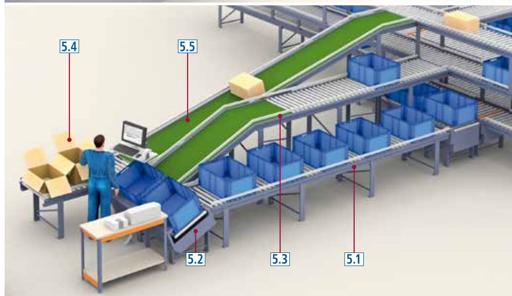
Details of picking position
