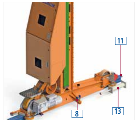
Lower track (11), hydraulic adjustment stop (13) and telemeter (8)
