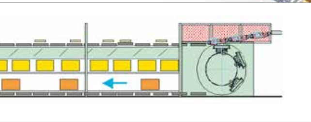
Section of a lateral view of the vertical sorter
