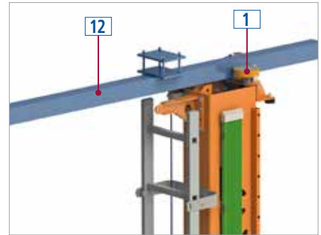
Top guide base (1) and upper track (12)
