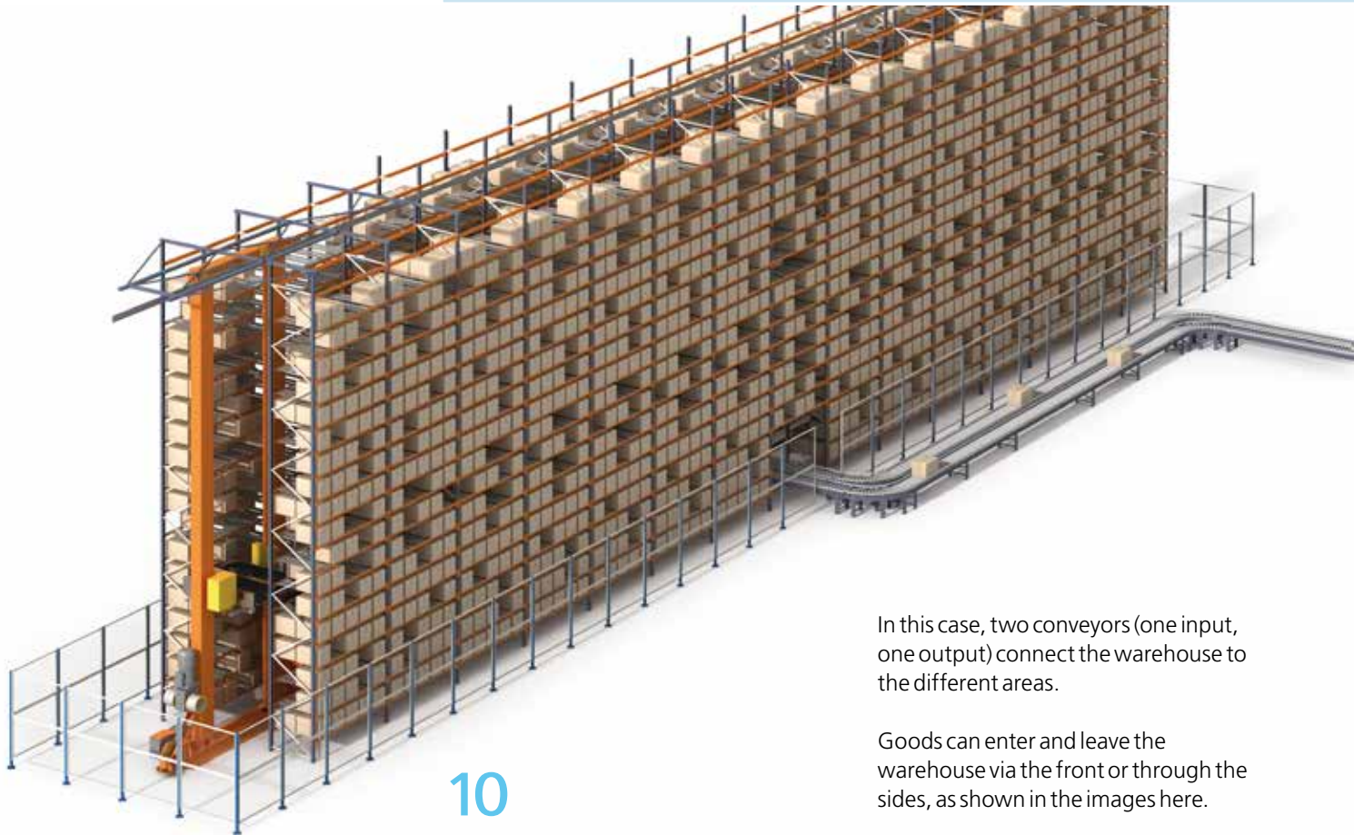
Automated warehouse for cardboard boxes with side entrance and exit.
